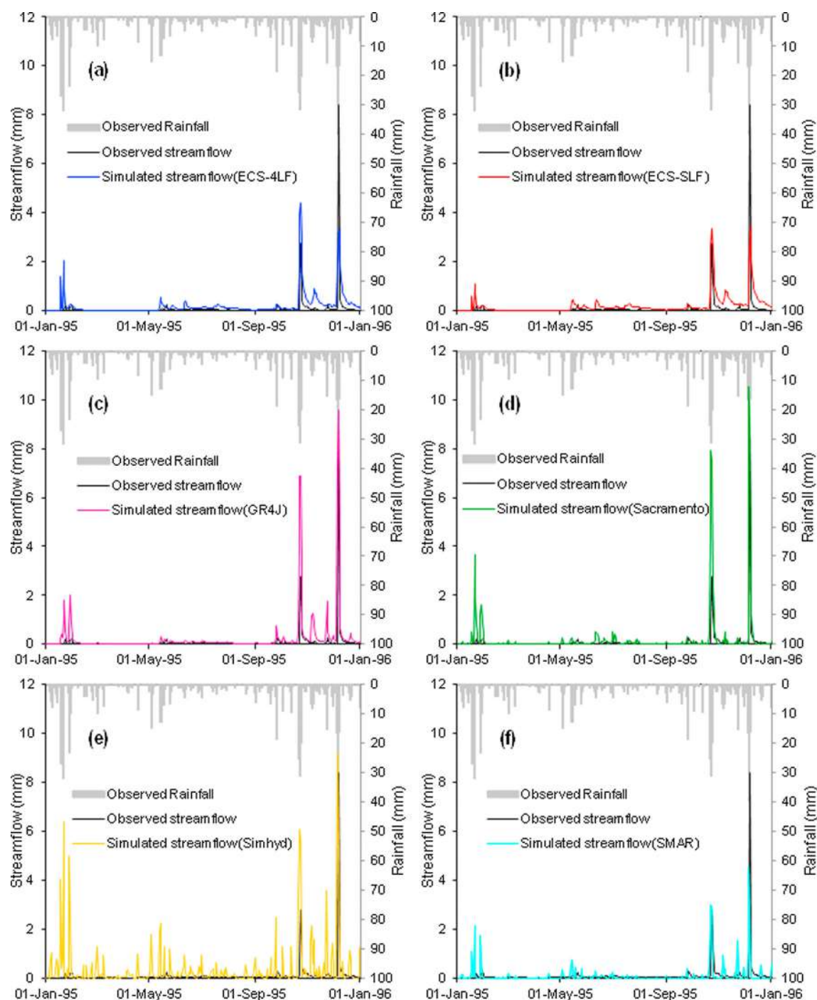
Fig. 4. Daily time series of observed and simulated streamflows from the a) ECS-4LF, b) ECS-SLF, c) GR4J, d) Sacramento, e) Simhyd and f) SMAR for the year 1995.
