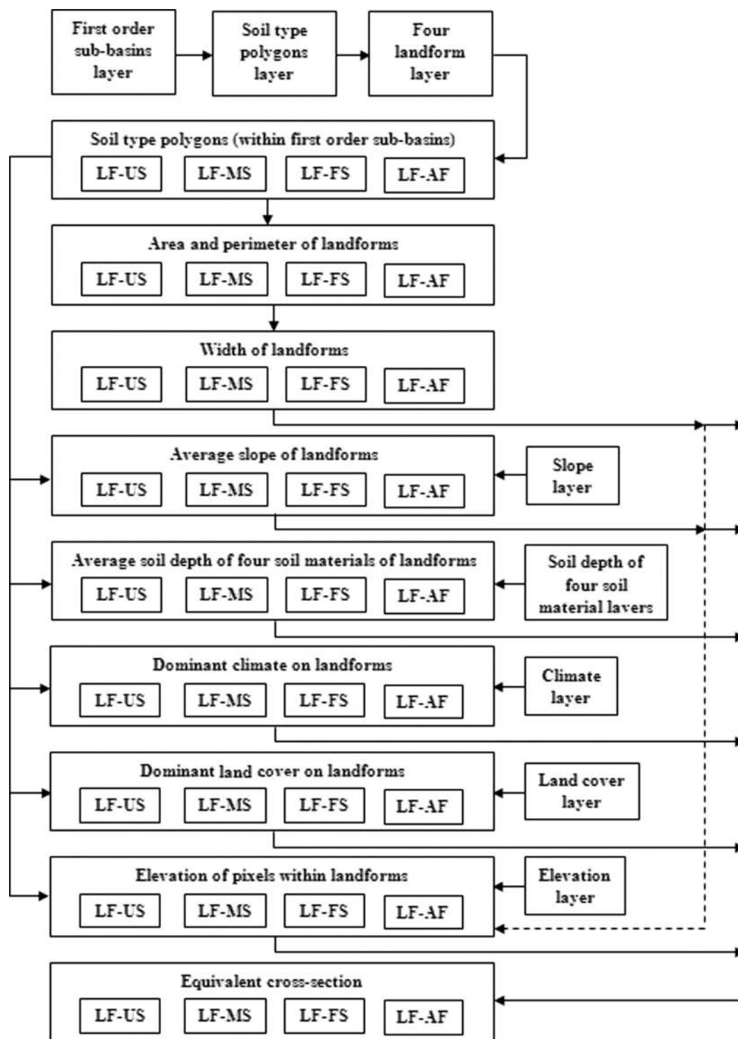
Fig. 3. Flow chart of the equivalent cross-section formulation. Landform-upslope (LF-US), Landform-midslope (LF-MS), Landform-footslope (LF-FS) and Landform-alluvial flats (LF-AF).
