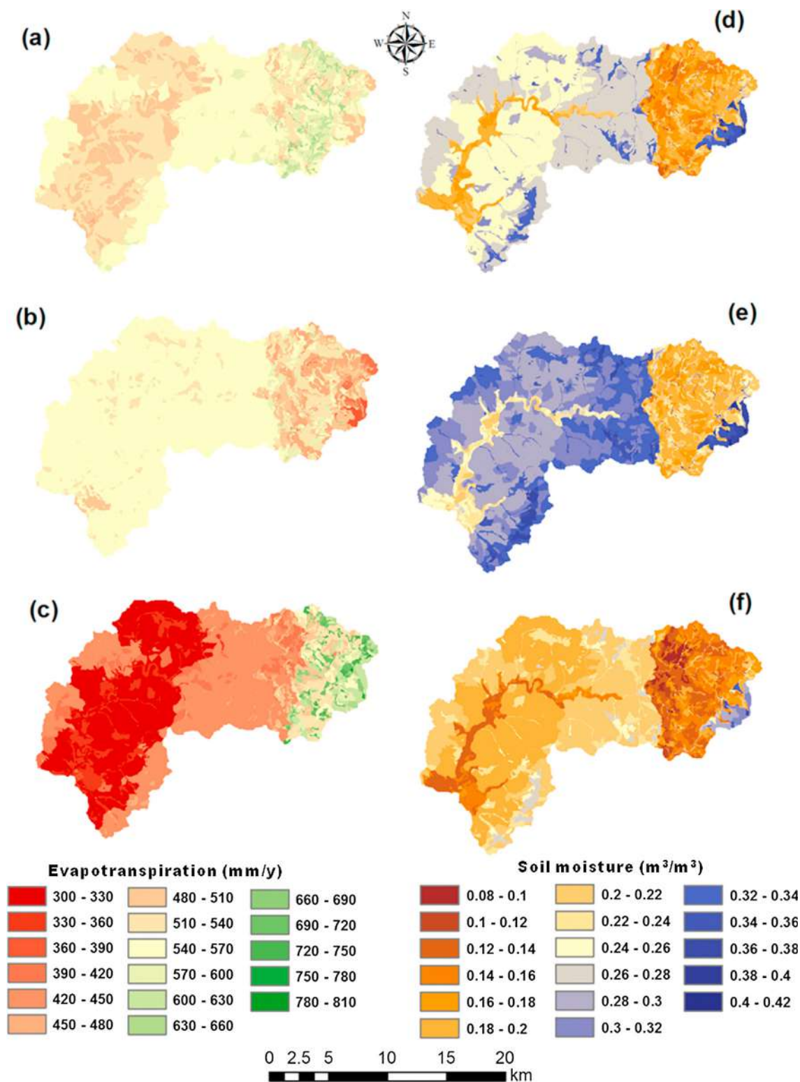
Fig. 7. Simulated actual evapotranspiration and soil moisture from the ECS-SLF approach for the McLaughlin catchment, a) average annual evapotranspiration, b) wet year (1978) evapotranspiration, c) dry year (1982) evapotranspiration, d) average soil moisture at surface soil layer for the whole study period (26 yr), e) wet year (1978) average soil moisture at surface soil layer and f) dry year (1982) average soil moisture at surface soil layer.
