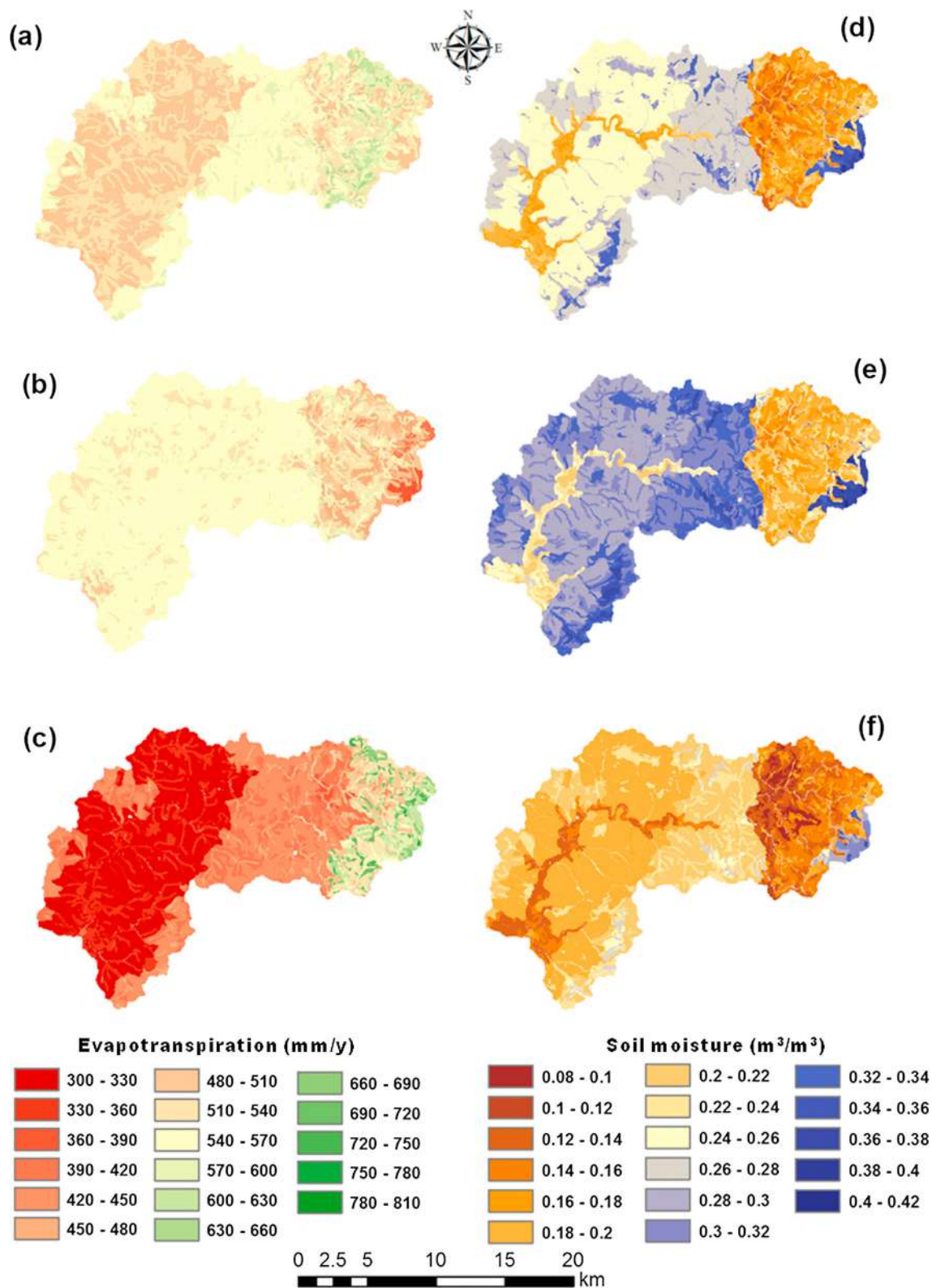
Fig. 6. Simulated actual evapotranspiration and soil moisture from the ECS-4LF approach for the McLaughlin catchment, a) average annual evapotranspiration, b) wet year (1978) evapotranspiration, c) dry year (1982) evapotranspiration, d) average soil moisture at surface soil layer for the whole study period (26 yr), e) wet year (1978) average soil moisture at surface soil layer and f) dry year (1982) average soil moisture at surface soil layer.
