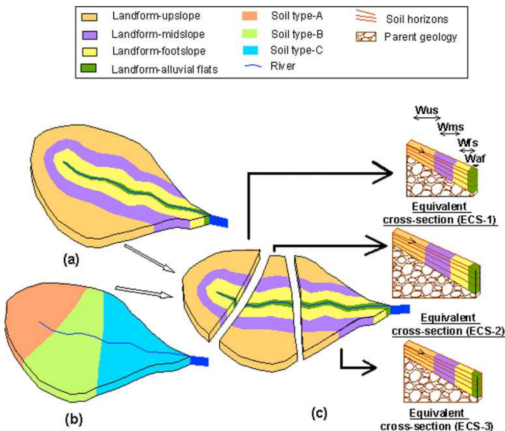
Fig. 2. Schematic of the equivalent cross-section modelling with four landforms approach, a) Four landforms are delineated for a first order sub-basin, b) Soil type map of a first order sub-basin is obtained, and c) First order sub-basin is divided into three sections based on soil type polygons. Equivalent cross-sections (ECS-1, ECS-2 and ECS-3) are formulated for each soil polygon and used in a 2-d distributed hydrologic modelling.
