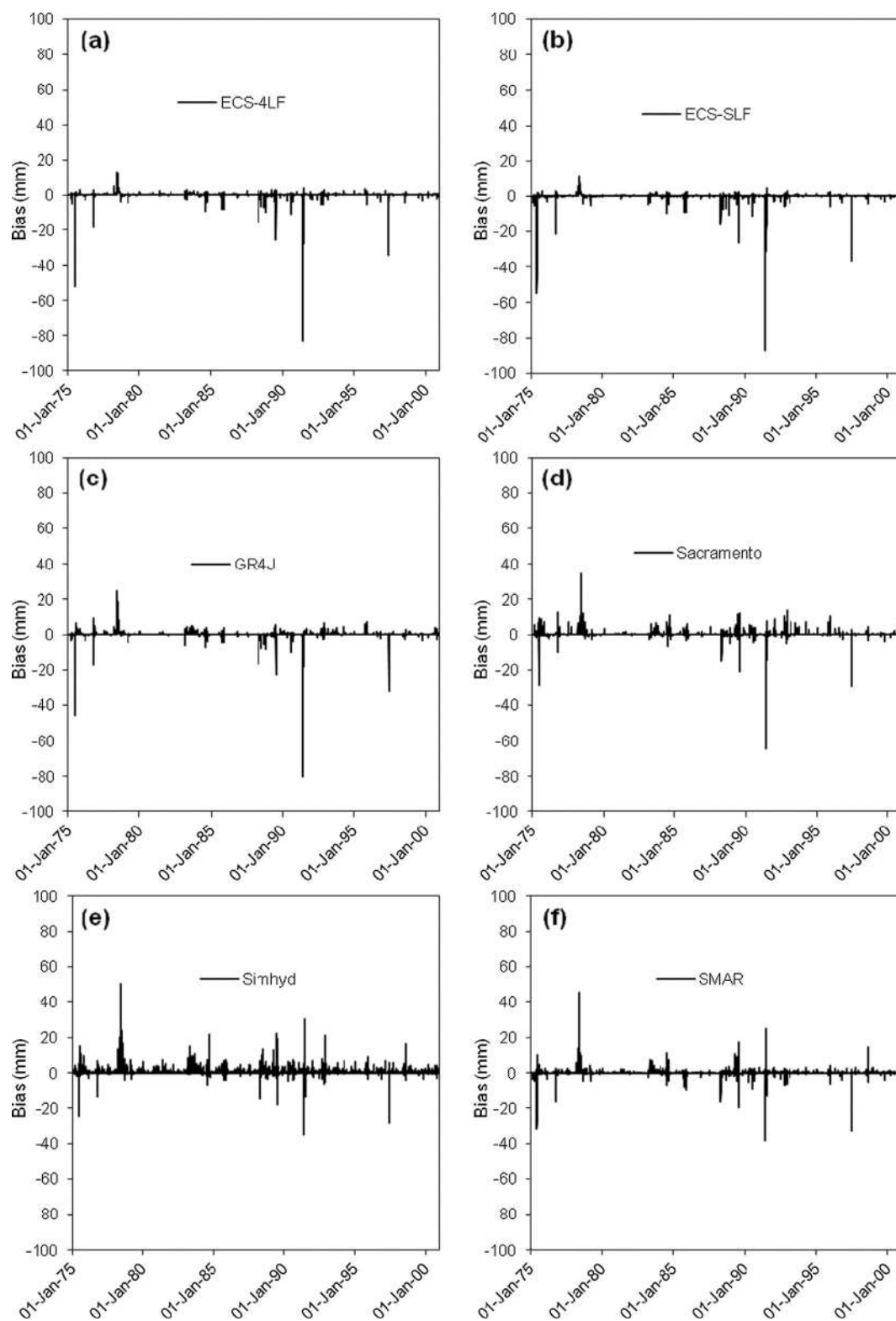
Fig. 5. Daily bias in streamflows simulated from a) ECS-4LF, b) ECS-SLF, c) GR4J, d) Sacramento, e) Simhyd and f) SMAR for the entire period (1975–2000).
