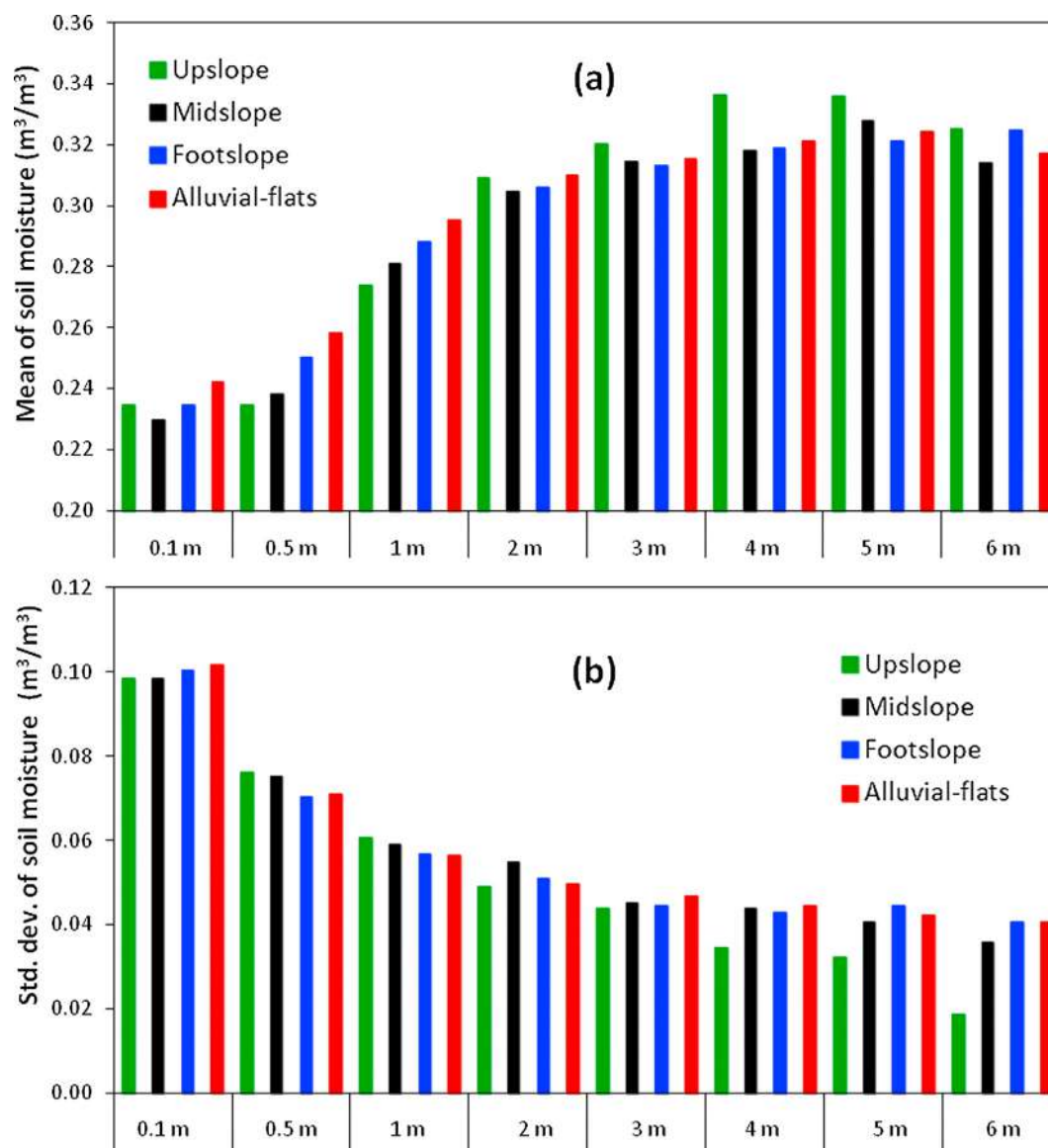
Fig. 12. Bar plots showing the a) mean and b) standard deviation of daily soil moisture across four landforms in the ECS-4LF approach at different soil depths for the McLaughlin catchment.
