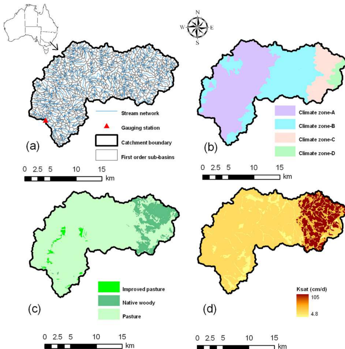
Fig. 1. a) Catchment map showing first order sub-basins and stream network, b) Climate zone map (A: < 600 mm/y; B: 600–750 mm/y; C: 750–900 mm/y and D: > 900 mm/y), c) Land cover map and d) Saturated Hydraulic Conductivity (Ksat) map of top soil horizon/material of the McLaughlin catchment.
