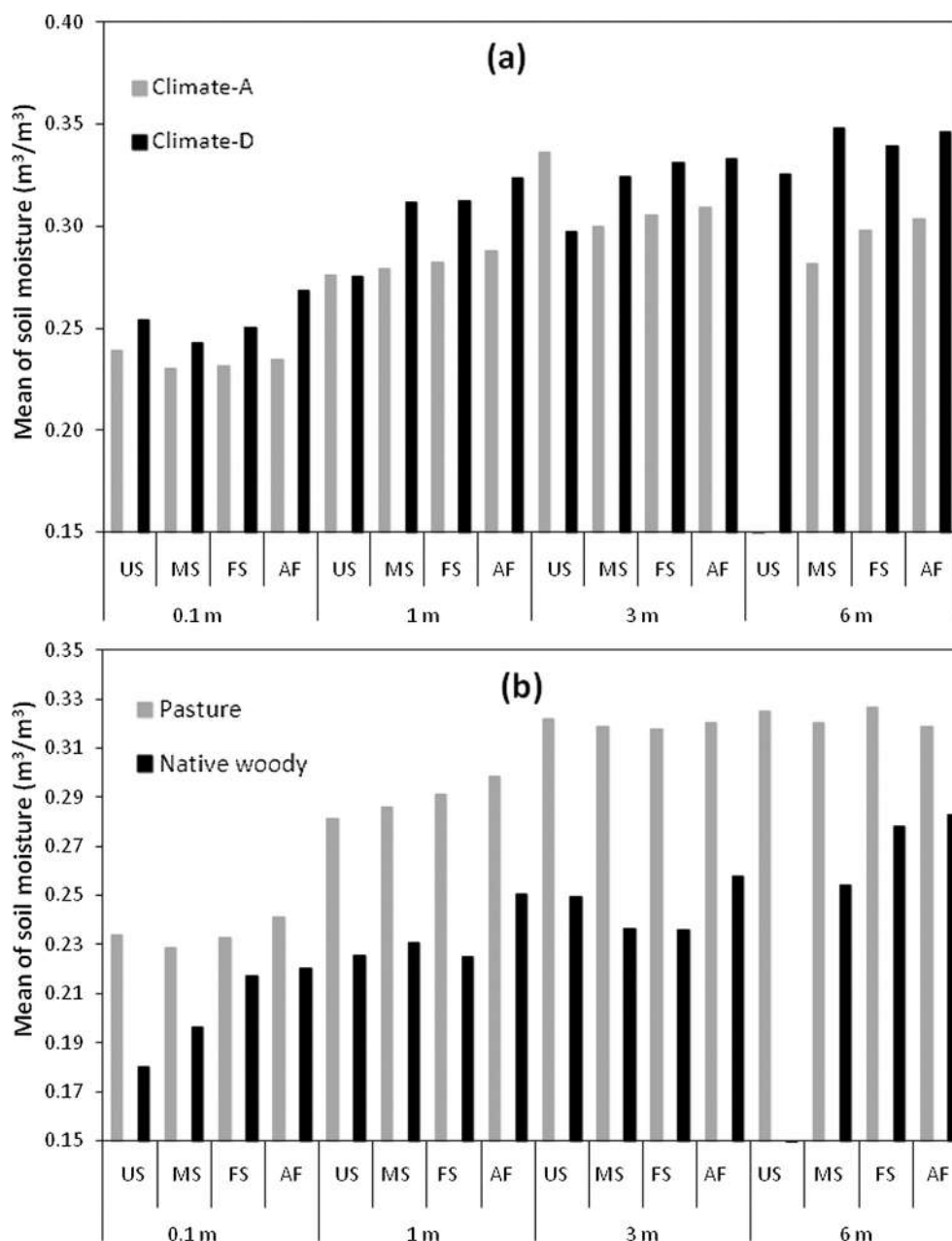
Fig. 13. Role of a) two extreme climatic zones (zone A dry & D wet) and b) land cover types (pasture and native woody) on vertical distribution of mean daily soil moisture at selected depths across four landforms within the McLaughlin catchment using the ECS-4LF approach. US, MS, FS and AF stand for landform-upslope, -midslope, -footslope and -alluvial-flats.
