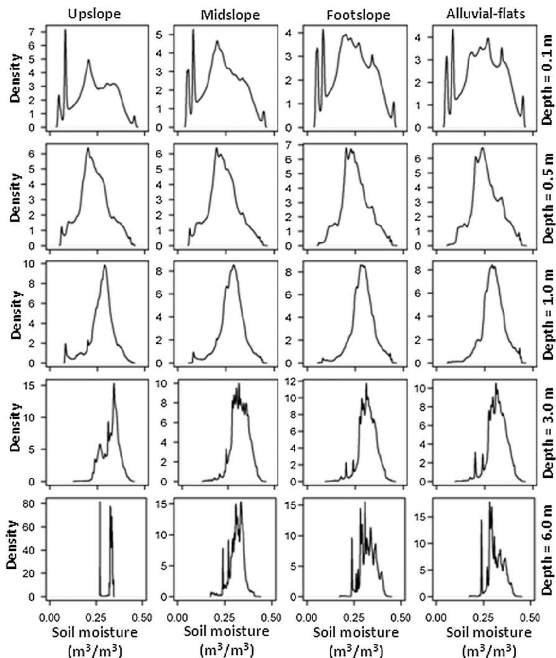
Fig. 11. Kernel density plots showing the distribution of daily soil moisture across four landforms at different soil depths in the ECS-4LF approach for the McLaughlin catchment.
