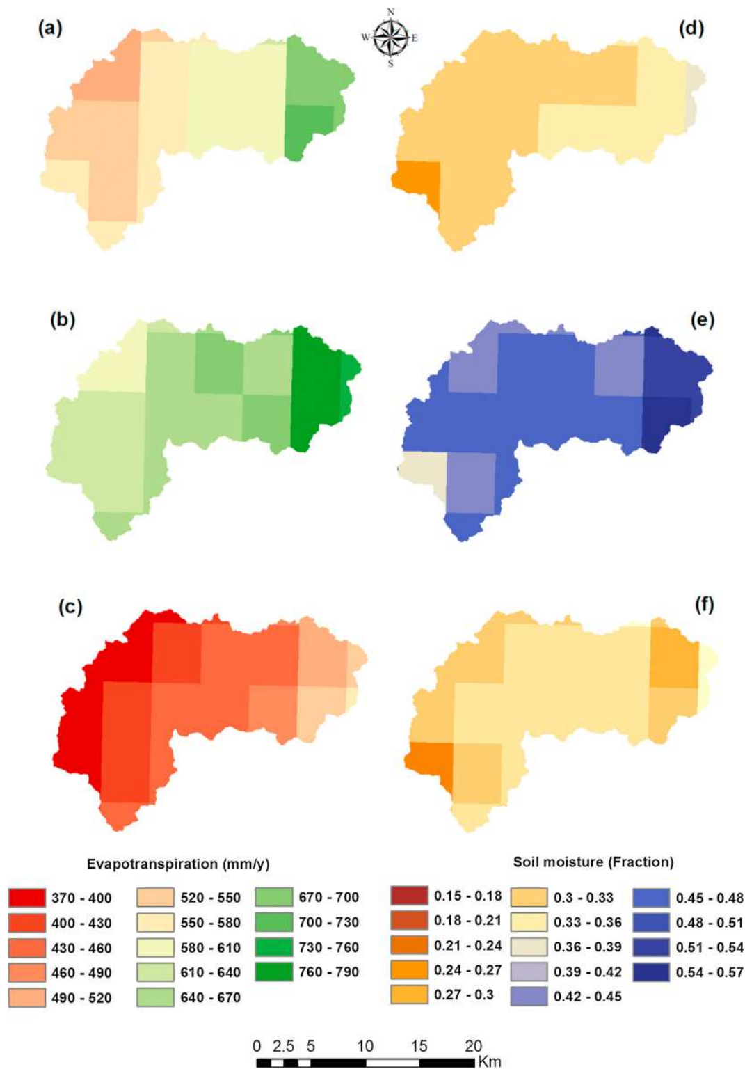
Fig. 9. Simulated actual evapotranspiration and soil moisture from the WaterDyn/AWAP model at 5 km × 5 km grid cells located partly or fully within the McLaughlin catchment, a) average annual evapotranspiration, b) wet year (1978) evapotranspiration, c) dry year (1982) evapotranspiration, d) average soil moisture at upper soil layer for the whole study period (26 yr), e) wet year (1978) average soil moisture at upper soil layer and f) dry year (1982) average soil moisture at upper soil layer.
