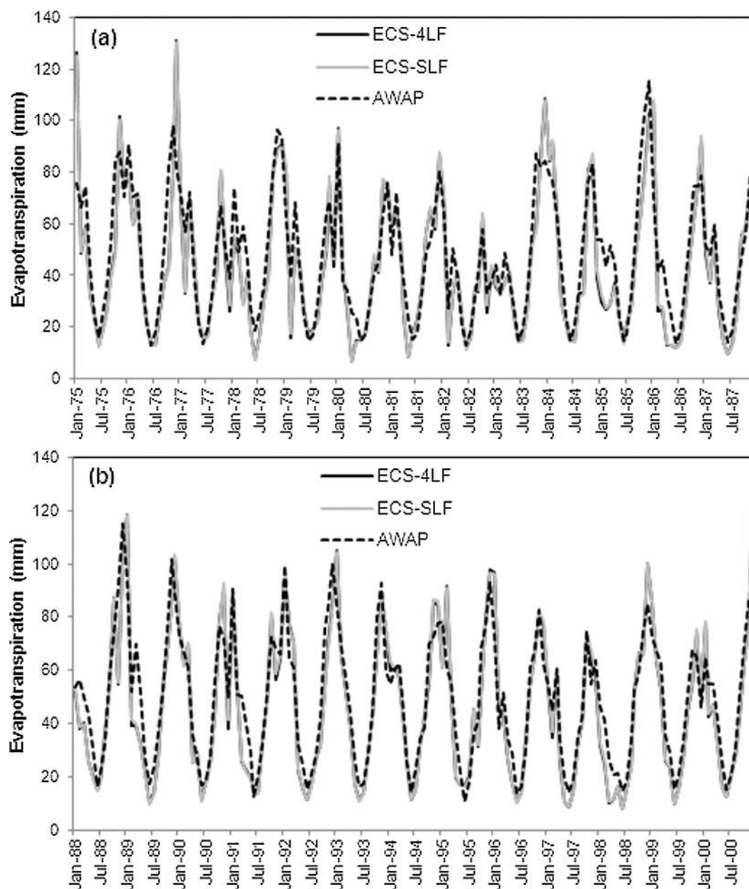
Fig. 8. Comparison of monthly simulated evapotranspiration from the ECS-4LF, ECS-SLF approaches and WaterDyn/AWAP model for the McLaughlin catchment for the period: a) 1975–1987 and b) 1988–2000. Note that the simulated evapotranspiration from the ECS-4LF and ECS-SLF are very close and black and grey lines overlap each other.
