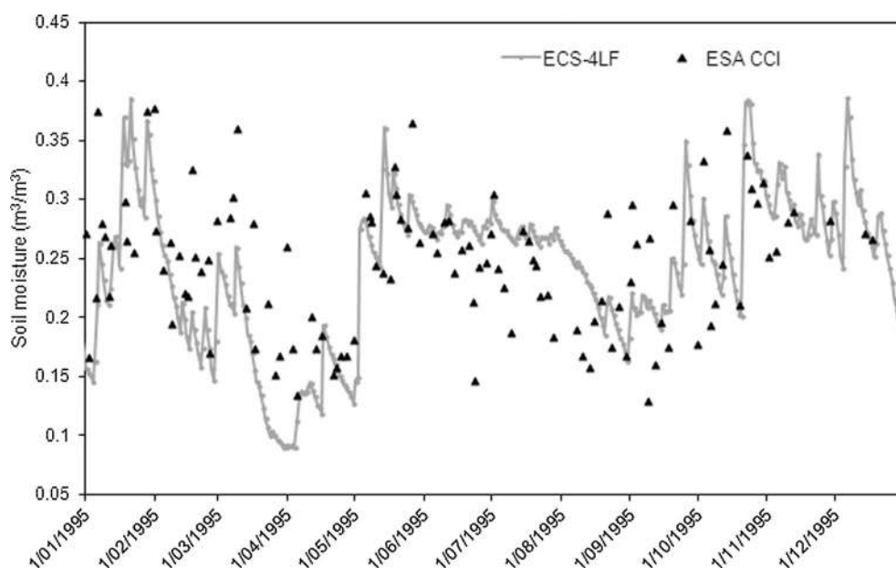
Fig. 10. Comparison of daily catchment average simulated soil moistures from the ECS-4LF approach with satellite derived ESA CCI daily catchment average soil moisture for the year 1995.
